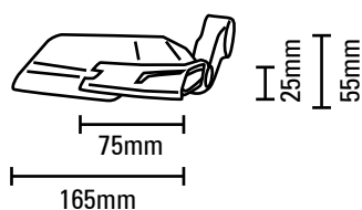
AERGO GP with Aerofoil fitted
