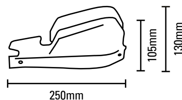
VPS with Wind Deflector fitted
